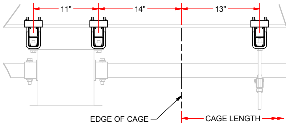
DETAIL B
